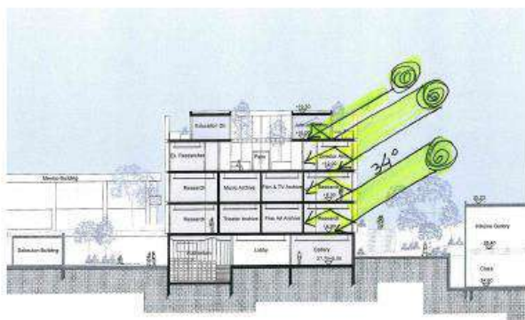
Sunlight Louvers - Winter- December 34°
