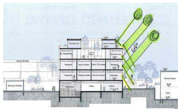
Sun Shading Louvers - Mid Season - September 64°
