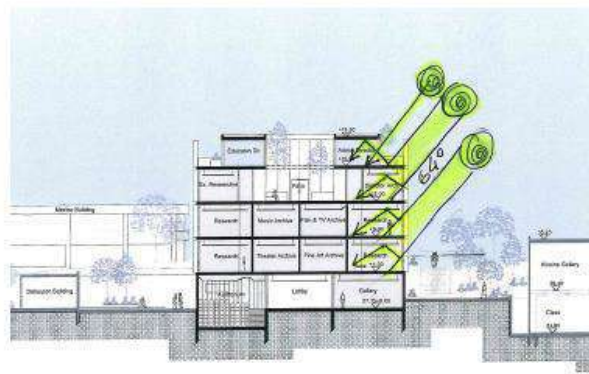
Sunlight Louvers - Mid Season - March 64°
