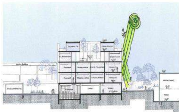
Sun Shading Louvers - Summer - June 81°
